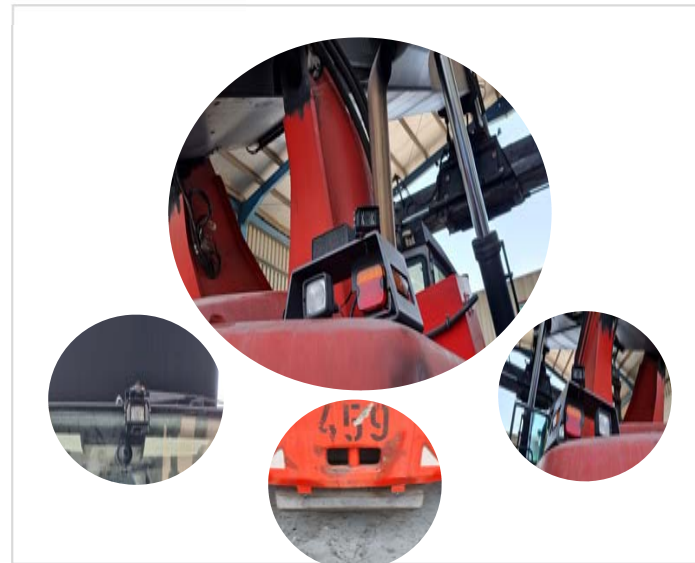
Reach stackers fitted with rear, front and cabin cameras and anti-collision sensors to the rear
