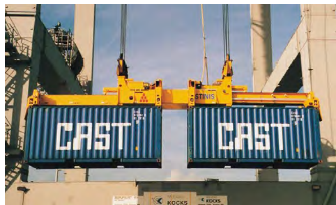
1996 STINIS LONG-TWIN® SPREADER
