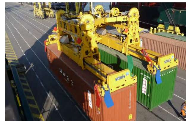
2005 STINIS SPLIT-HEADBLOCK®
