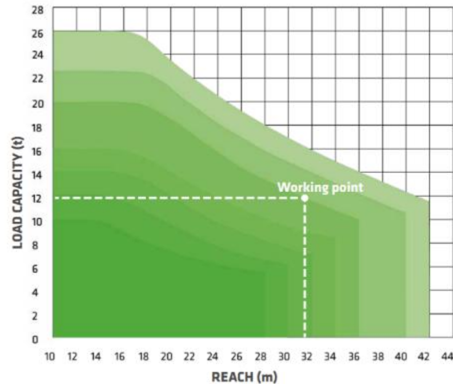
Performance curves of the EQ G Balancer range
